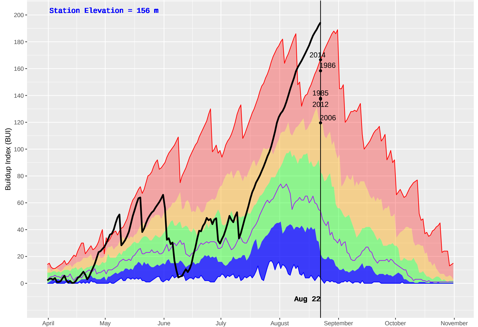
WOSS CAMP (21) : Historical (1970–2016) and Current (2018) Daily Buildup Index (BUI)
