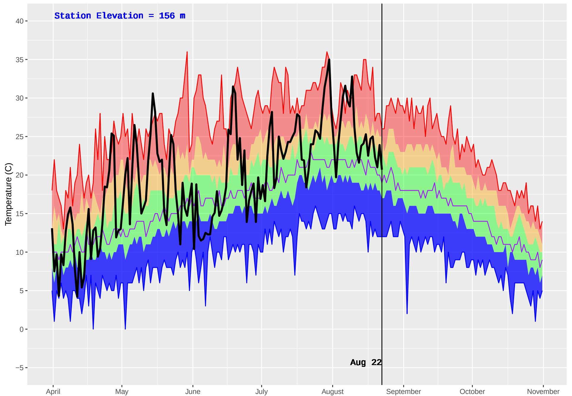
WOSS CAMP (21) : Historical (1970–2016) and Current (2018) Daily Temperature
